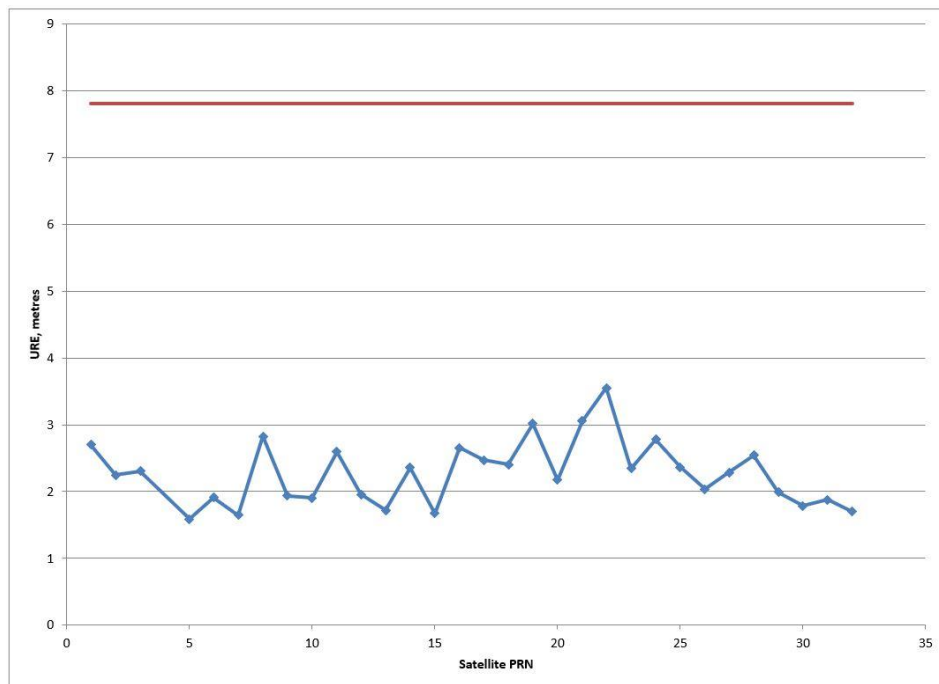
Figure 3-1: Constellation URE (95%) for Reporting Period
