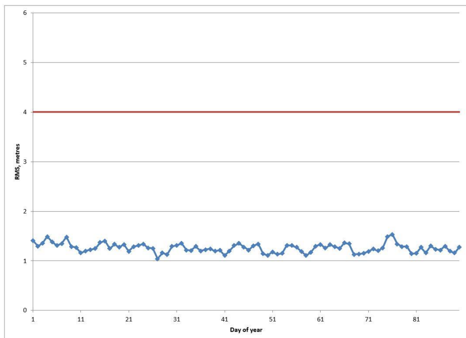
Figure 3-2: Constellation RMS URE for Reporting Period
