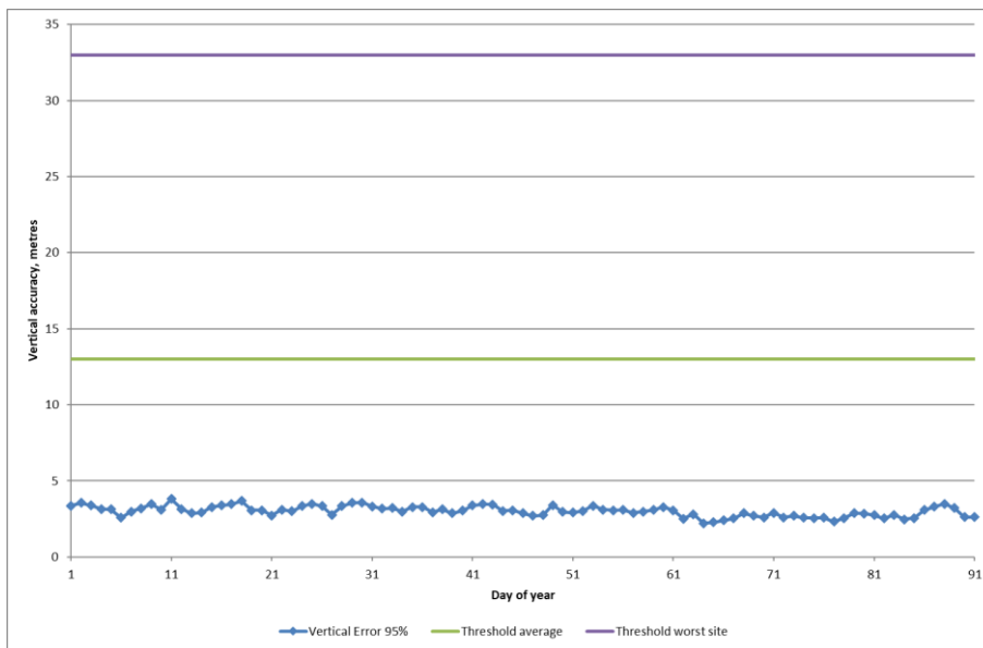
Figure 5-1: Daily Vertical Accuracy Values for GPS L1/L2 solution
