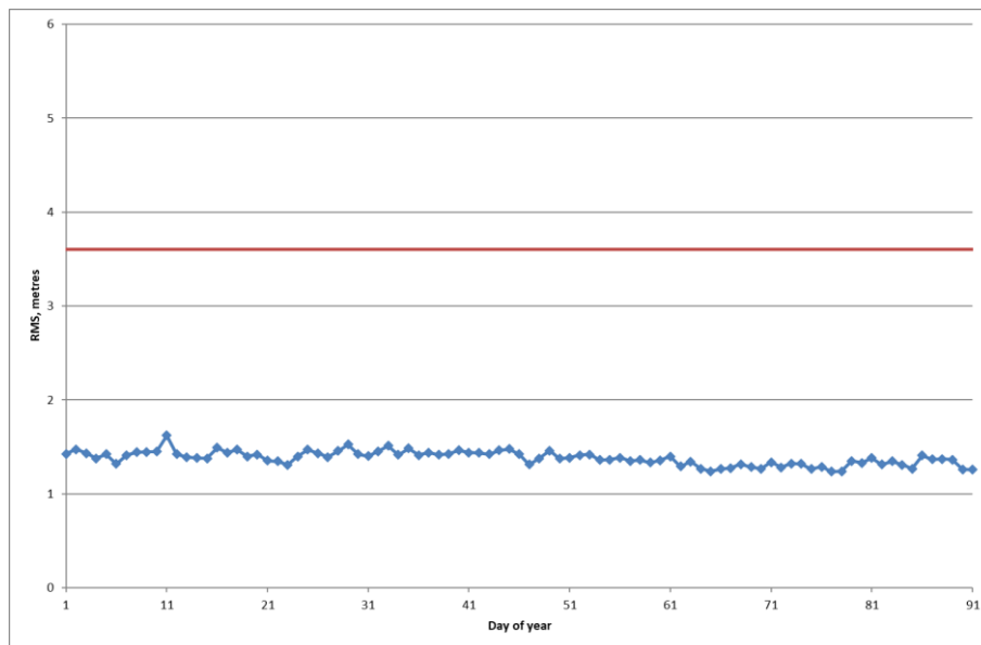
Figure 5-2: Constellation RMS URE (dual frequency) for Reporting Period
