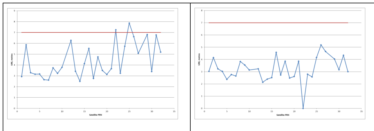
Figure 5-1: Constellation URE (95%) for Reporting Period (left) and Period after 24 th January (right)
