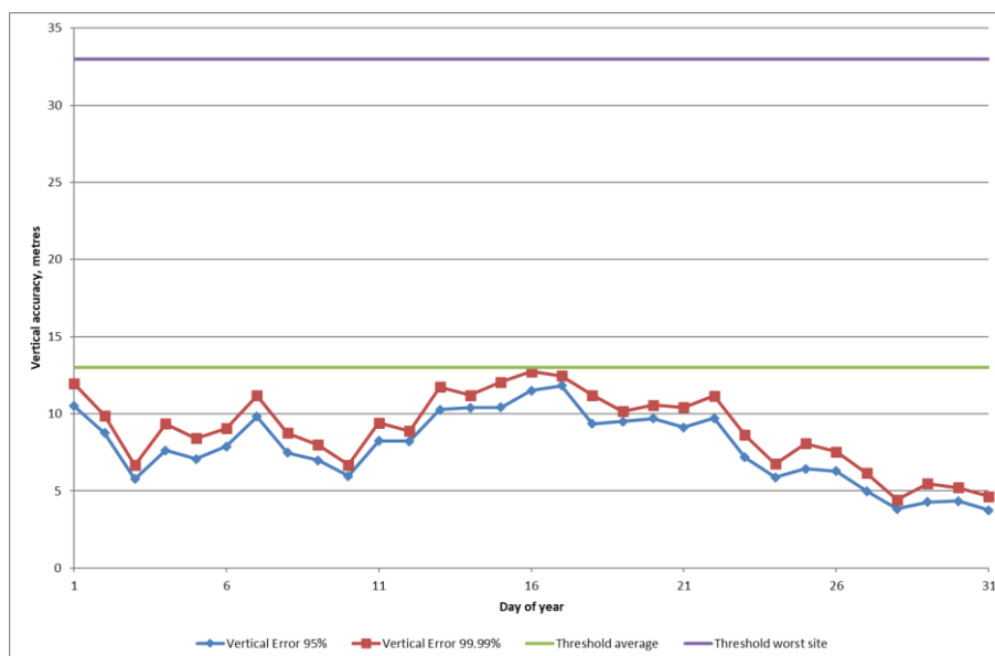
Figure 5-3: Daily Vertical Accuracy Values for January for GPS L1 solution at MLG1
