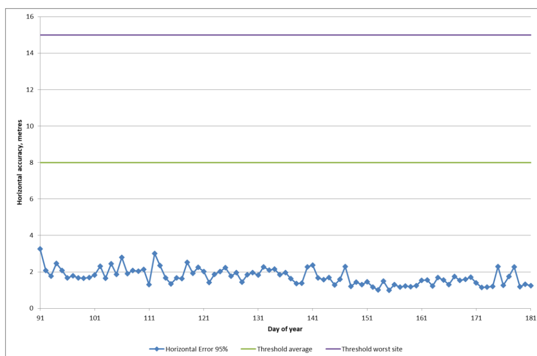
Figure 3-7: Daily Horizontal Position Accuracy (95%) for Reporting Period
