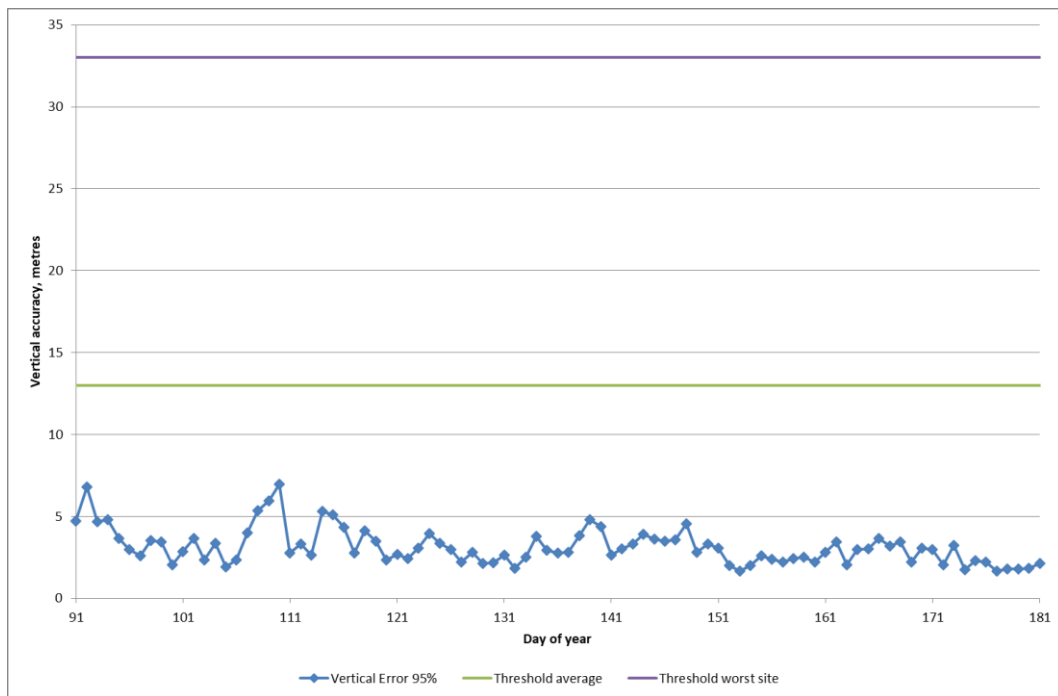
Figure 3-8: Daily Vertical Position Accuracy (95%) for Reporting Period
