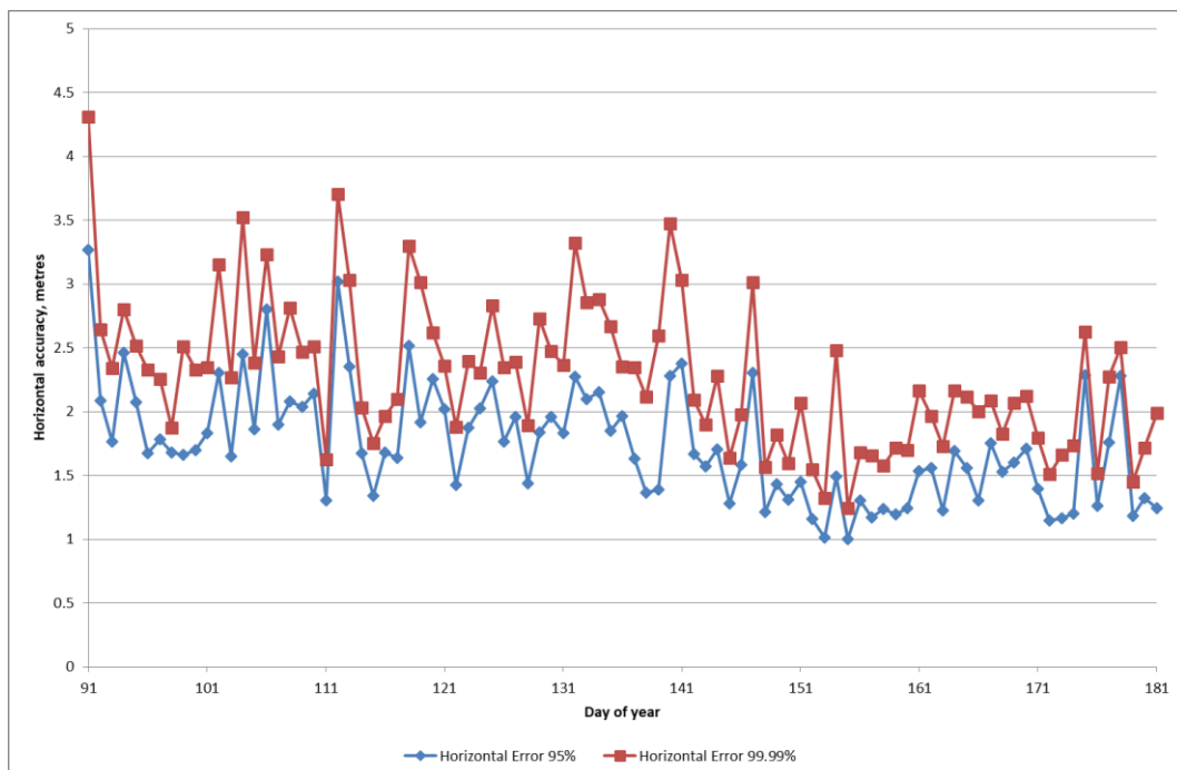
Figure 3-9: Daily Horizontal Position Accuracy (99.99%) for Reporting Period
