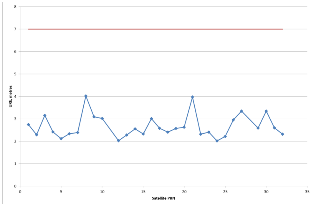
Figure 3-1: Constellation URE (95%) for Reporting Period
