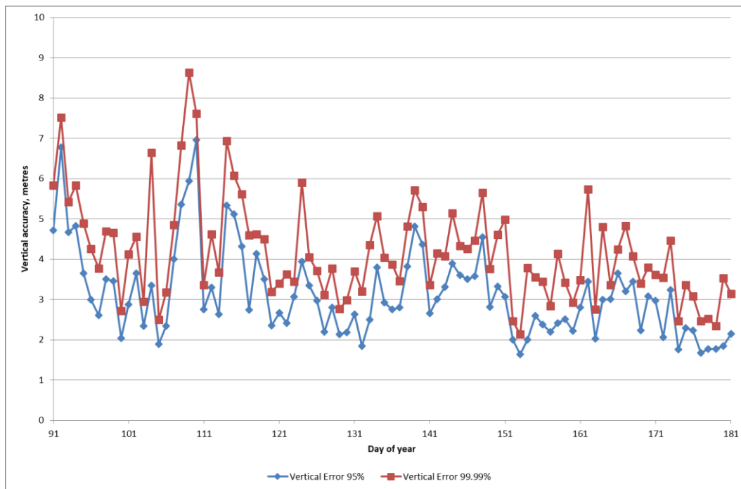
Figure 3-10: Daily Vertical Position Accuracy (99.99%) for Reporting Period
