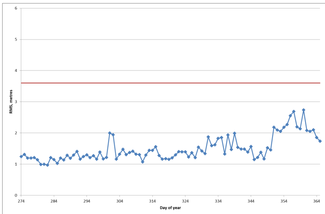
Figure 3-2: Constellation RMS URE for Reporting Period
