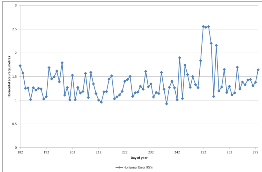
Figure 3-3: Horizontal Position Accuracy (95%) for Monitoring Period
