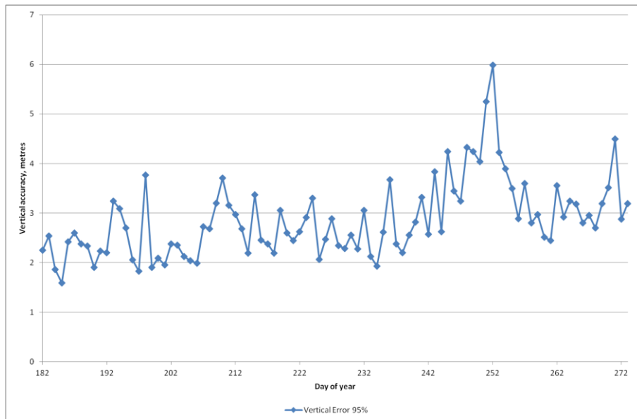
Figure 3-4: Vertical Position Accuracy (95%) for Monitoring Period
