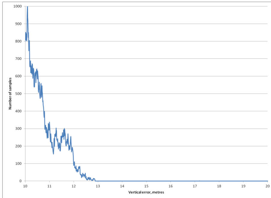
Figure 3-4: Vertical Error Distribution above 10m for Monitoring Period
