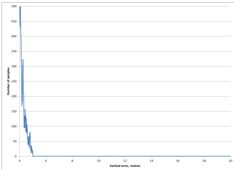
Figure 3-4: Vertical Error Distribution above 4m for Monitoring Period
