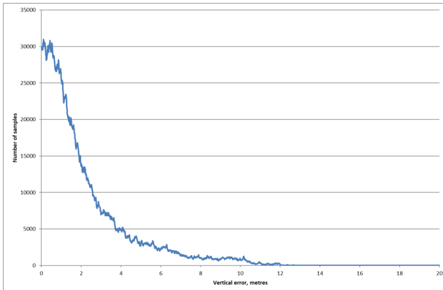
Figure 3-2: Vertical Error Distribution for Monitoring Period
