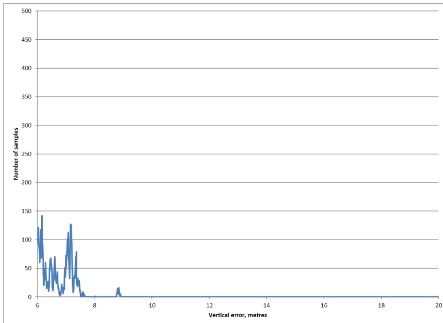
Figure 3-4: Vertical Error Distribution above 6m for Monitoring Period
